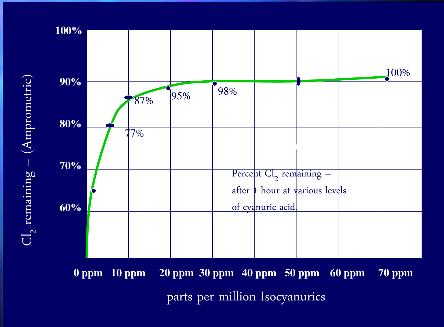
Figure 13-2: Stabilized chlorine “staying power”
