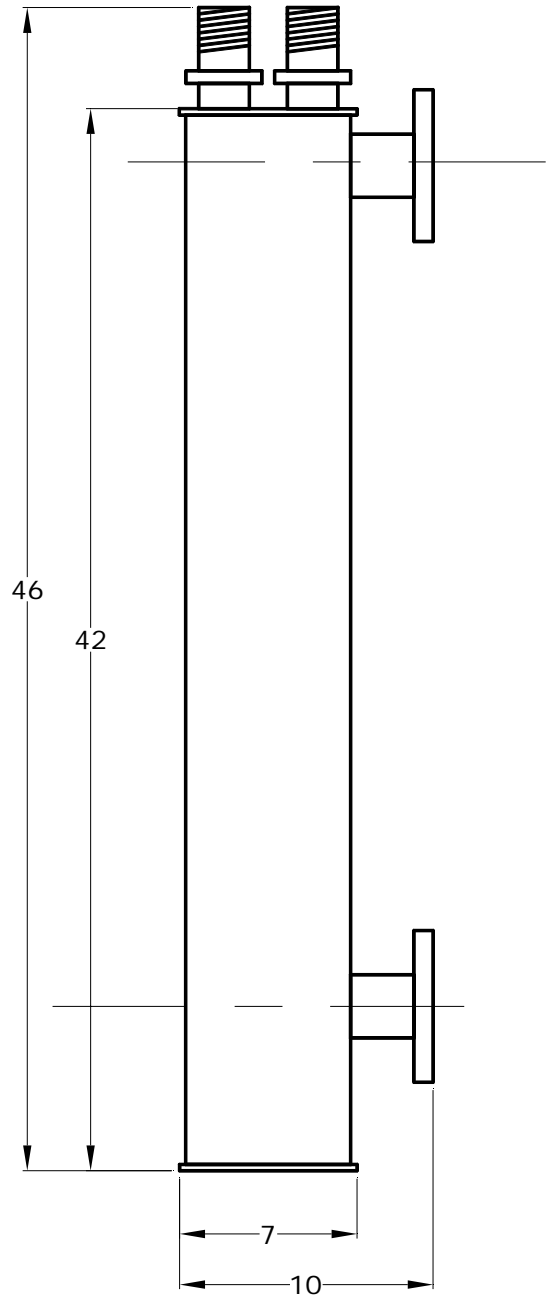
Flanges Same Side
