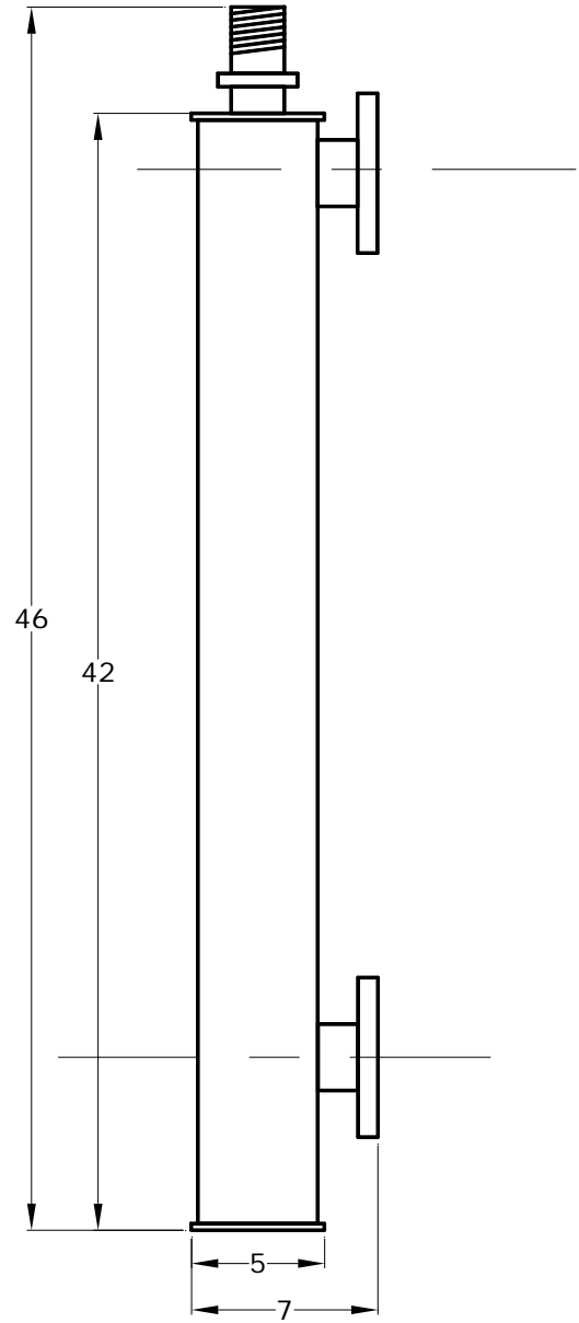
Flanges Same Side
