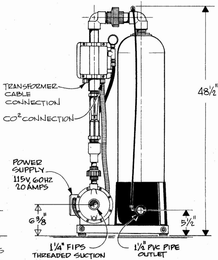
REAR ELEVATION
