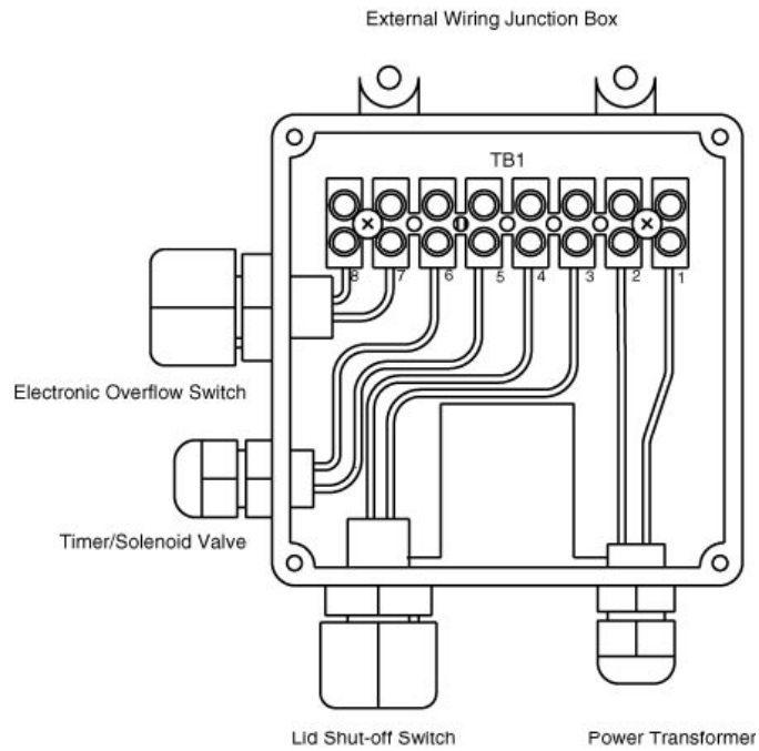
Figure 1 - Junction Box Terminator Strip
